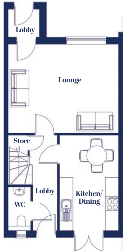
Lobby 1.4m x 1.2m Lounge 4.9m x 3.9m Kitchen/Dining 2.6m x 4.6m
